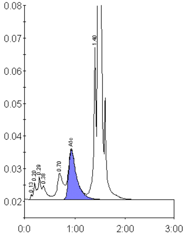
Peak table - ID: 10576295
